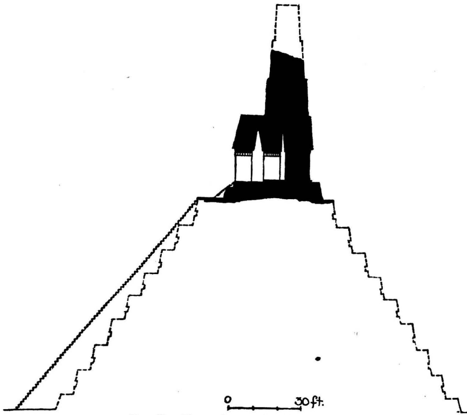
FIG. 42.—TIKAL: Cross-section of Temple III.
