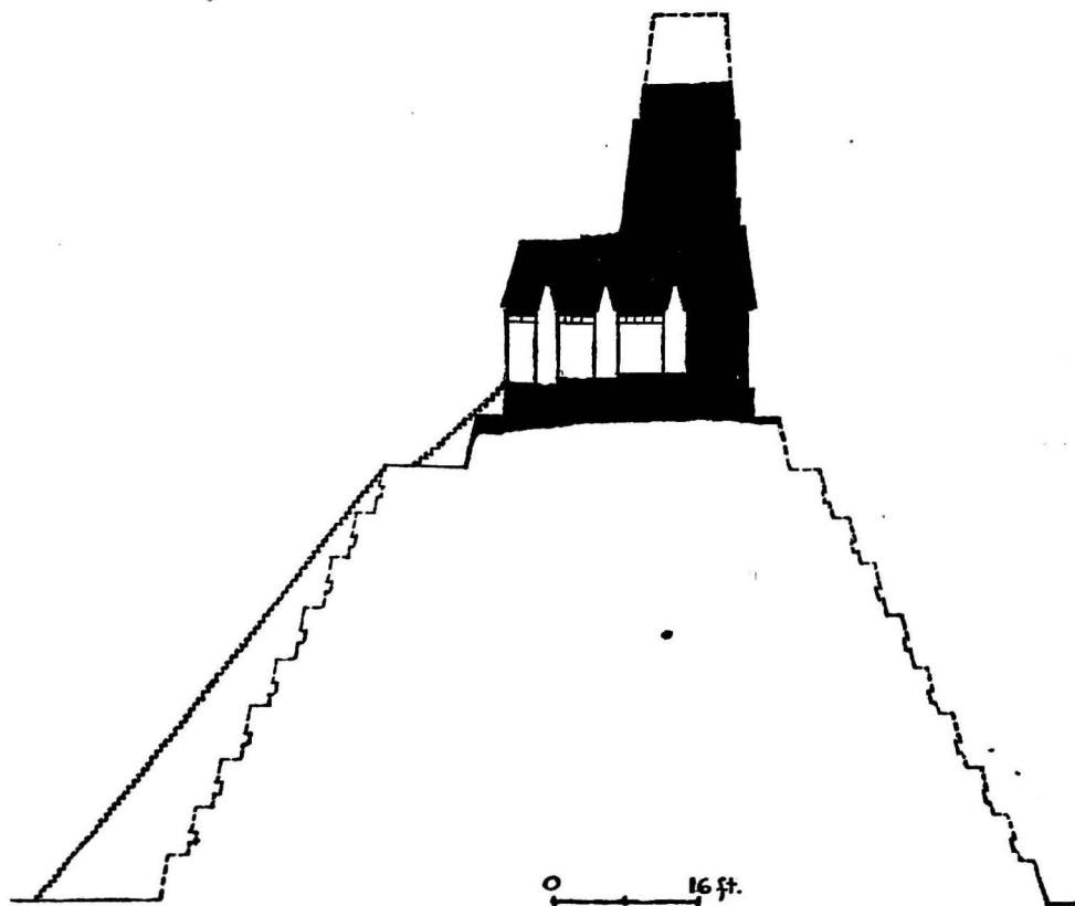
FIG 30. — TIKAL: Cross-section of Temple I.
