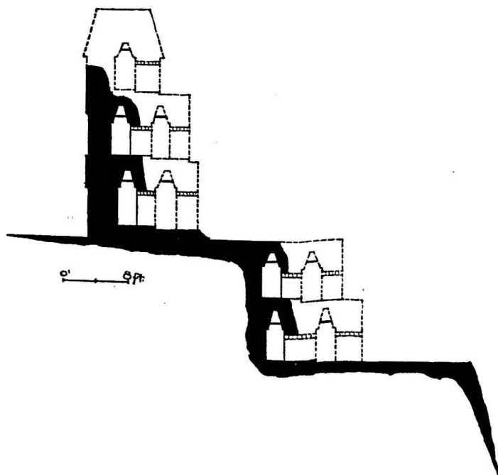
FIG. 24. — TIKAL: Cross-section of Structure 10.
