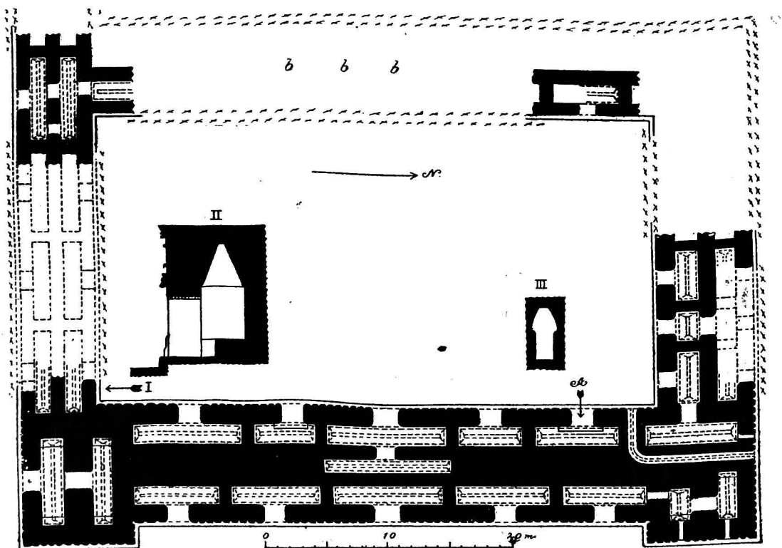
FIG. 1. — TIKAL: PLAN AND SECTIONS OF PALACE OF THE FAÇADES WITH VERTICAL GROOVES. I. Head in frieze. II. Cross Section of inner room (A). III. Cross Section of northeastern passage. b b b. High mounds of debris formed by fallen edifice of two stories.
