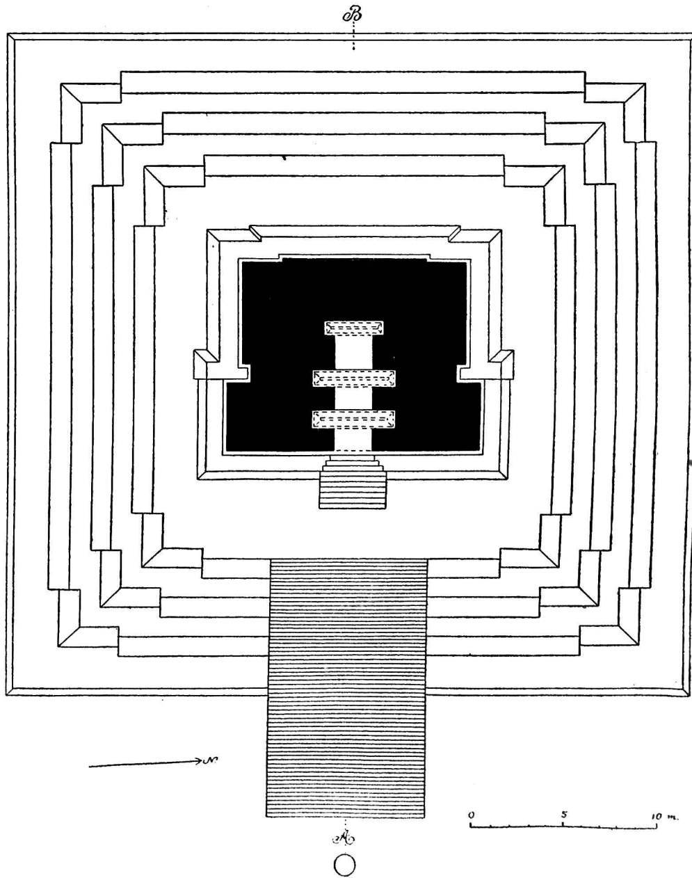
FIG. 5. — TIKAL: Plan of Temple II.
