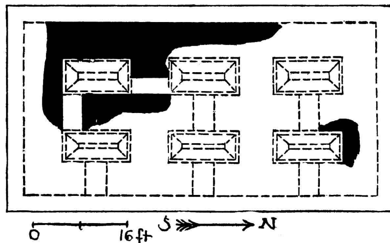
FIG. 46. — TIKAL: Plan of Structure 89.
