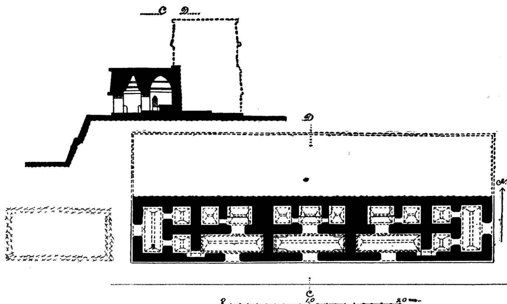
FIG. 2. — TIKAL: PLAN AND SECTION OF THE PALACE WITH REAR CHAMBERS AND GREAT STONE BENCHES.
