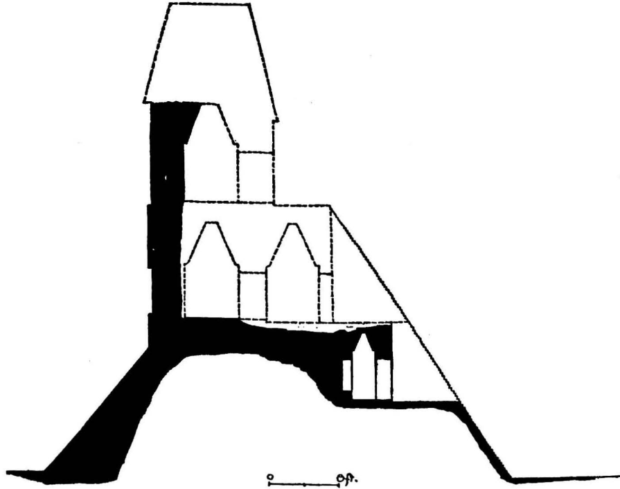
FIG. 21 — TIKAL: Cross-section of Structure 27.
