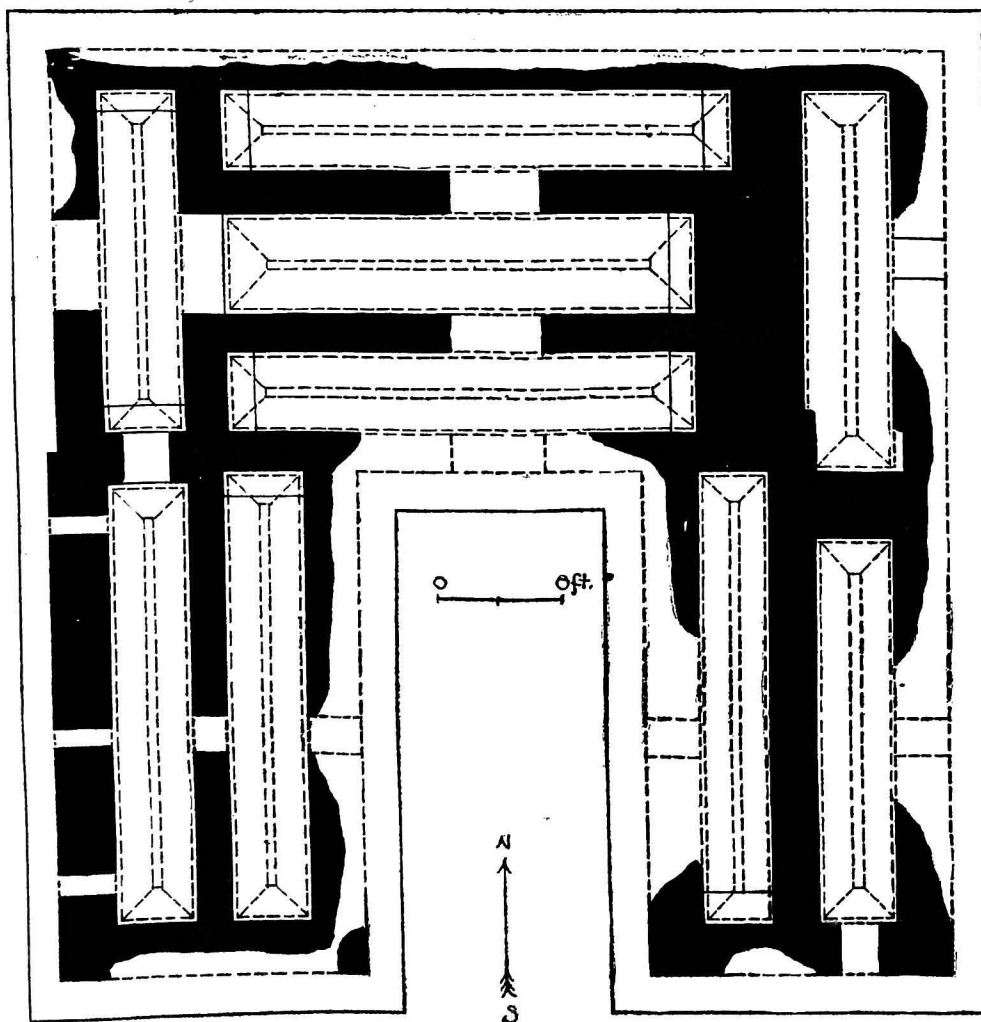
FIG. 28. — TIKAL: Plan of Structure 18.
