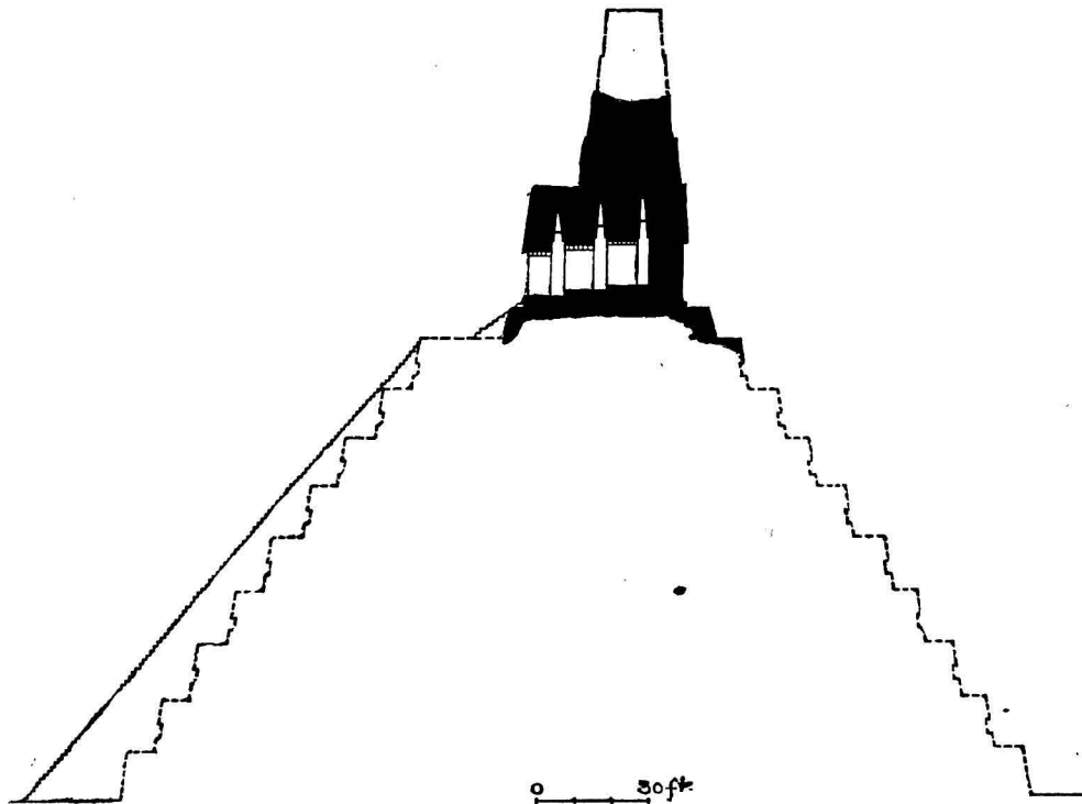
FIG. 45. — TIKAL: Cross-section of Temple IV.
