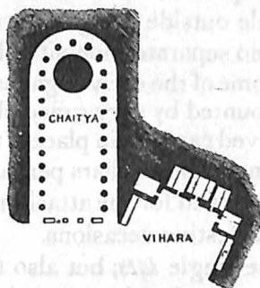
Plan of chaitya -cave and vihāra , Bhaja. After Fergusson.
